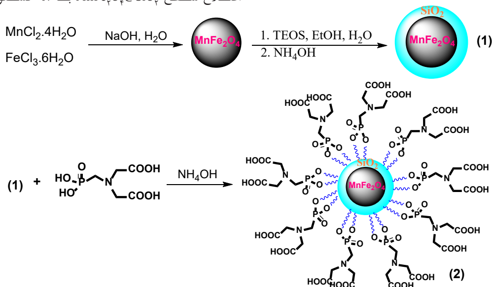
Schematic 1. Synthesis process of \text{MnFe}_2\text{O}_4@\text{SiO}_2 core-shell magnetic nanoparticles functionalized with N-phosphonomethylaminodiacetic acid ( \text{MnFe}_2\text{O}_4@\text{SiO}_2 PMIDA)
