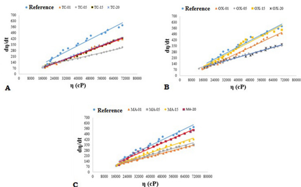
Figure 4 - Changes in d\eta/dt versus viscosity for binder systems (HTPB-DOS-TDI) containing three tetracycline (A), oxalic acid (B) and maleic acid (C) at ^{\circ}\text{C} 40
