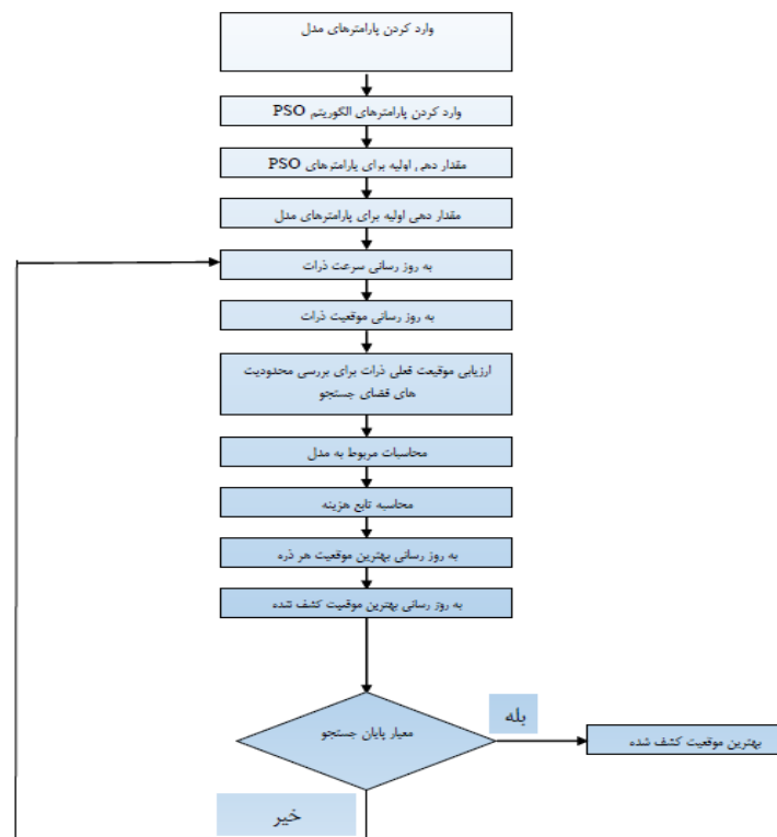
Fig. A1. Scheme of PSO algorithm, used to minimize the cost function (the sum of the squared weighted errors) and obtain kinetic parameters
