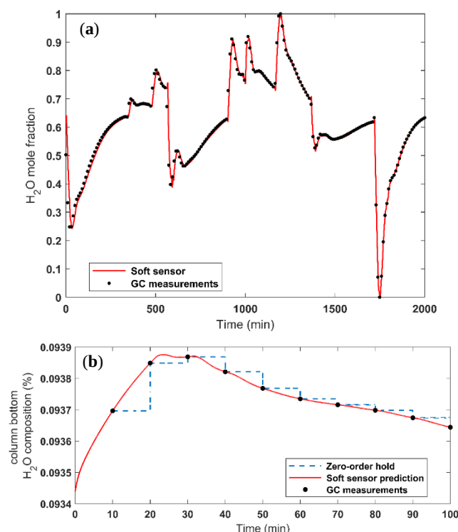
Figure 13 a) Comparison of analyzer measurements and FFNN model predicted water mole fraction, b) Comparison of PV14 variable measurement estimation using the ZOH method and soft sensor
